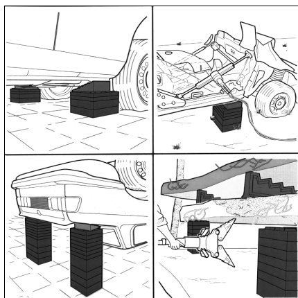
TYPE B CHOCKING SETS
