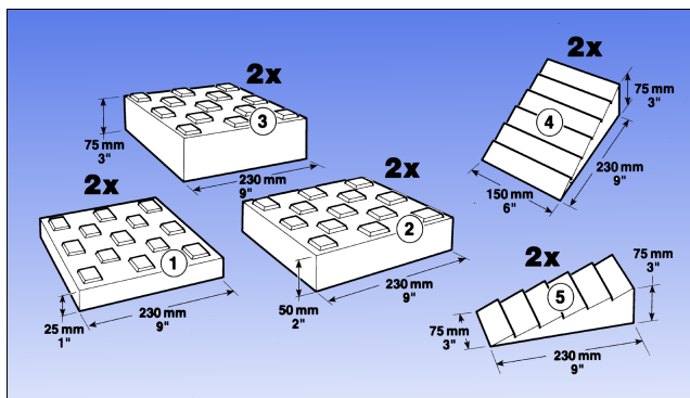
TYPE B CHOCKING SETS
